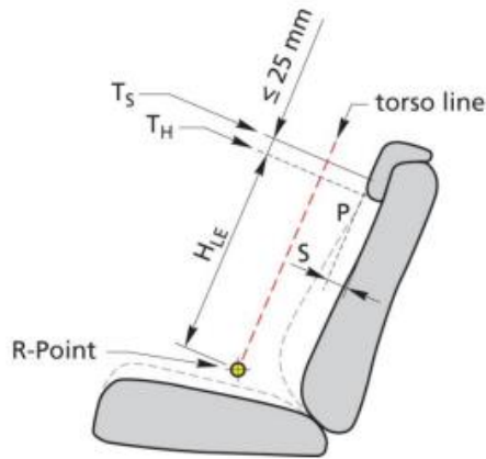
Figure 6 Discomfort metric geometric requirements
