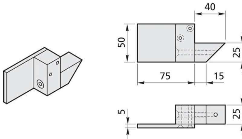
Figure 9 Discomfort metric gauge design example (all dimension in mm)
