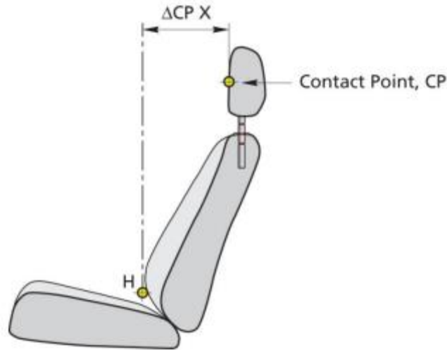
Figure 3 Calculation of backset
