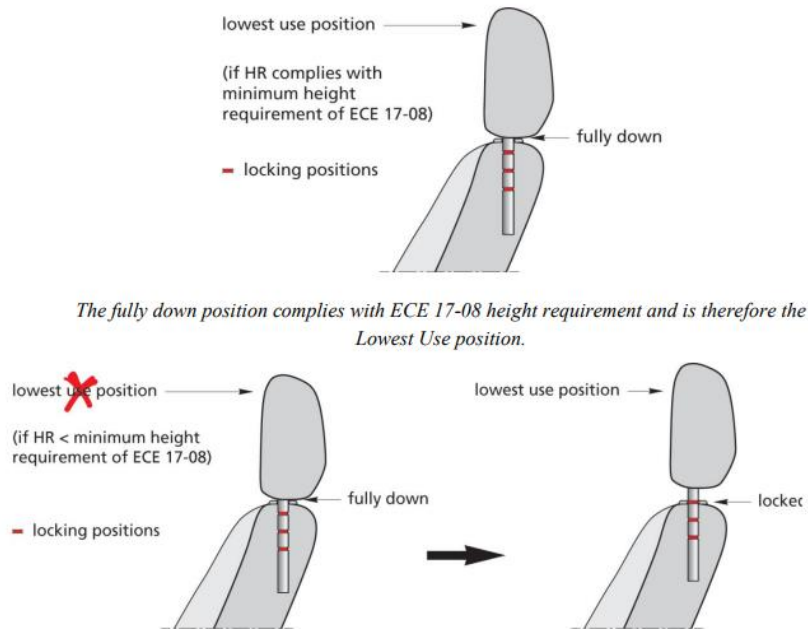
Figure 8 Examples of setting lowest use position
