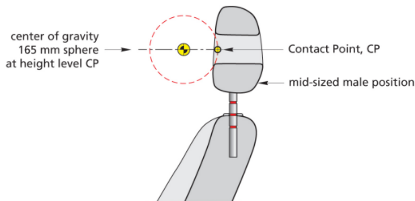
Figure 1 Definition of CP in the presence of a gap in the head restraint
