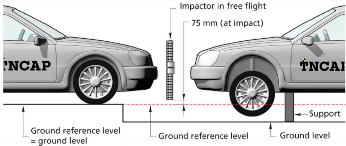
Figure 26: Legform to Bumper tests
