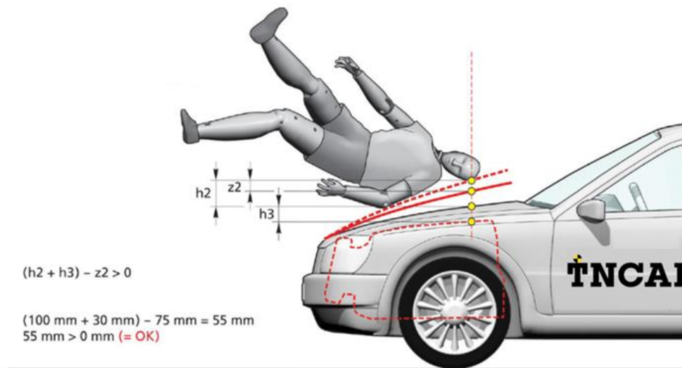
Figure 4: Bonnet deflection total clearance requirement
