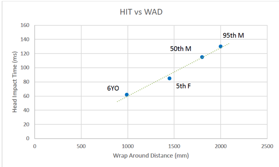
Figure 25: WAD vs HIT
