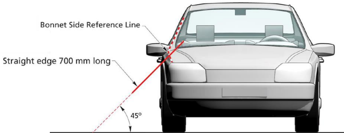
Figure 5: Determination of the bonnet side reference lines
