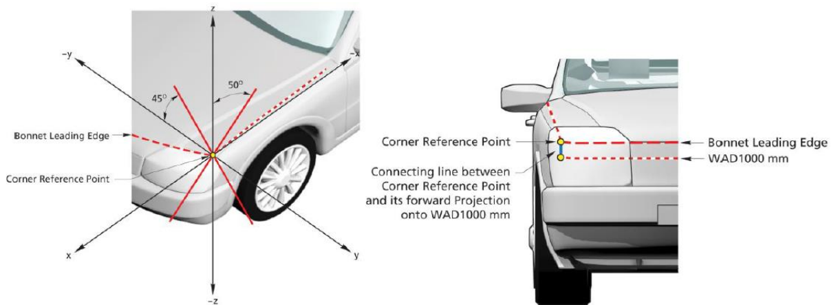
Figure 11: Determination of the corner reference point
