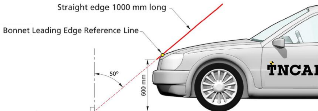
Figure 6: Determination of the Bonnet Leading Edge Reference Line
