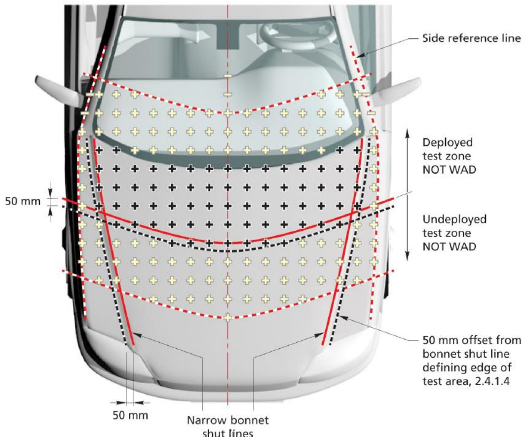
Figure 2: Area to meet low speed requirement
