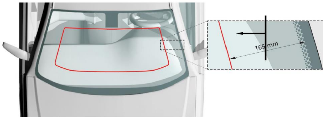
Figure 23: Windscreen periphery measurement
