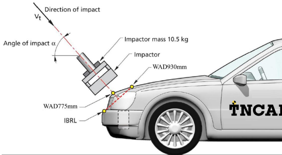
Figure 29: Upper Legform to WAD775mm Test
