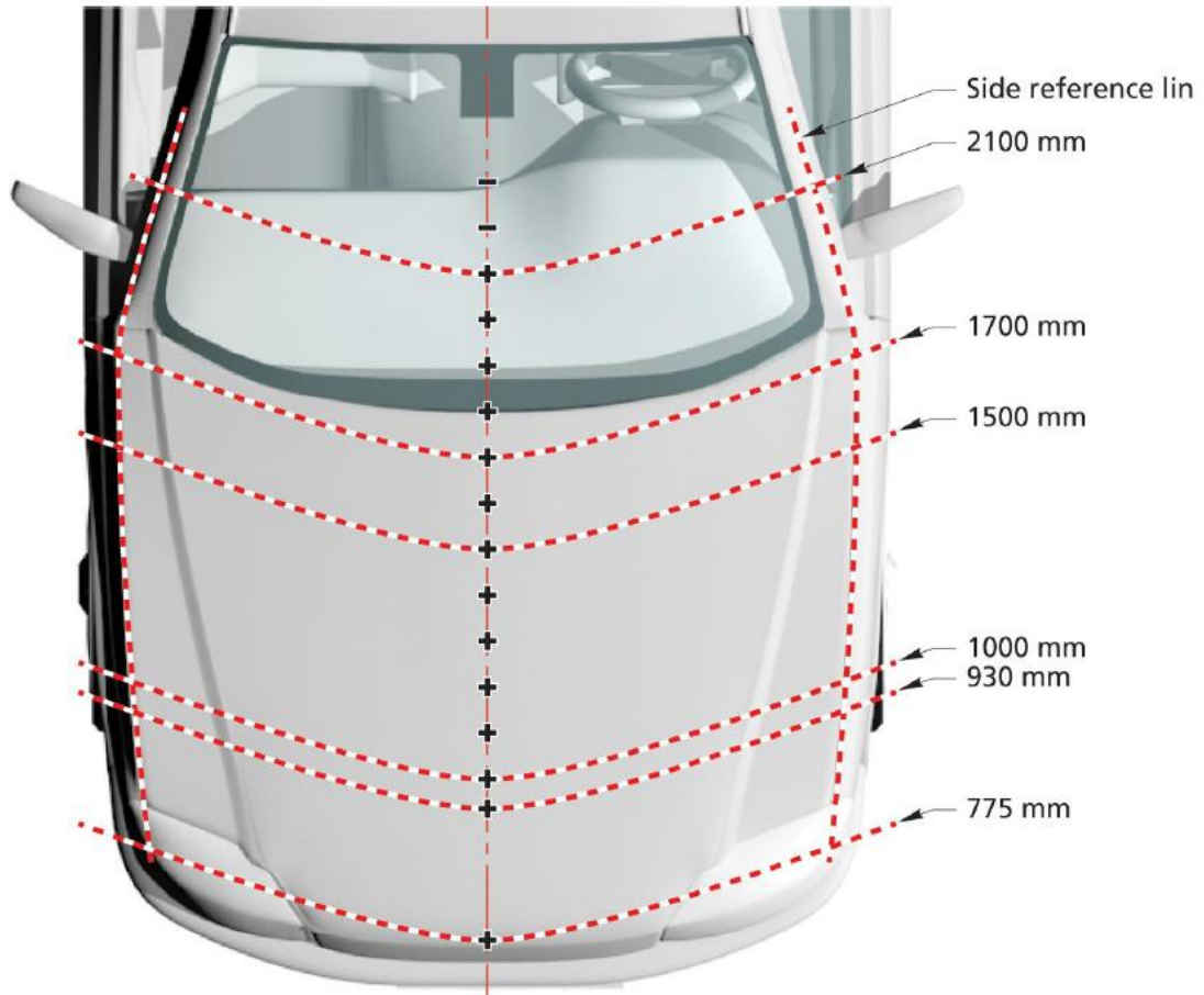
Figure 10: Headform test area
