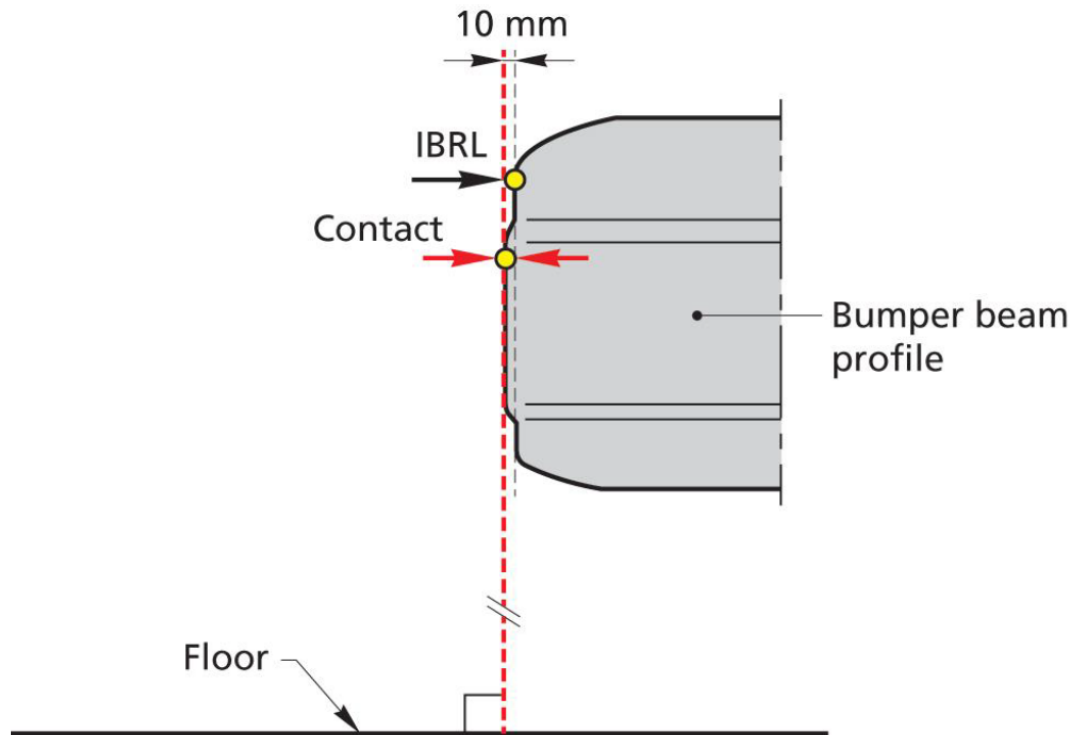
Figure 15: Marking IBRL height
