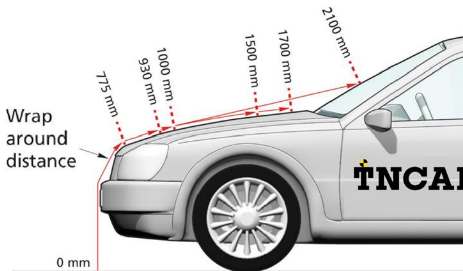
Figure 9: Marking wrap around lines
