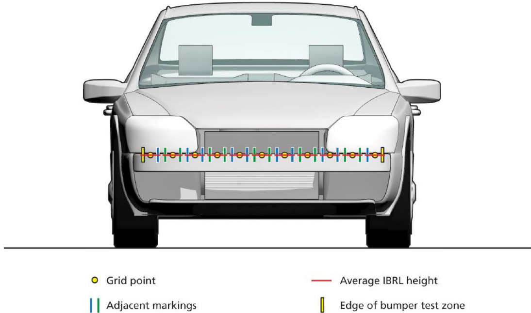
Figure 16: IBRL height at 100mm intervals
