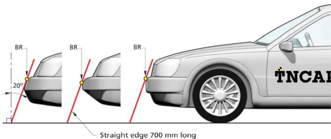
Figure 12: Determination of upper bumper reference line
