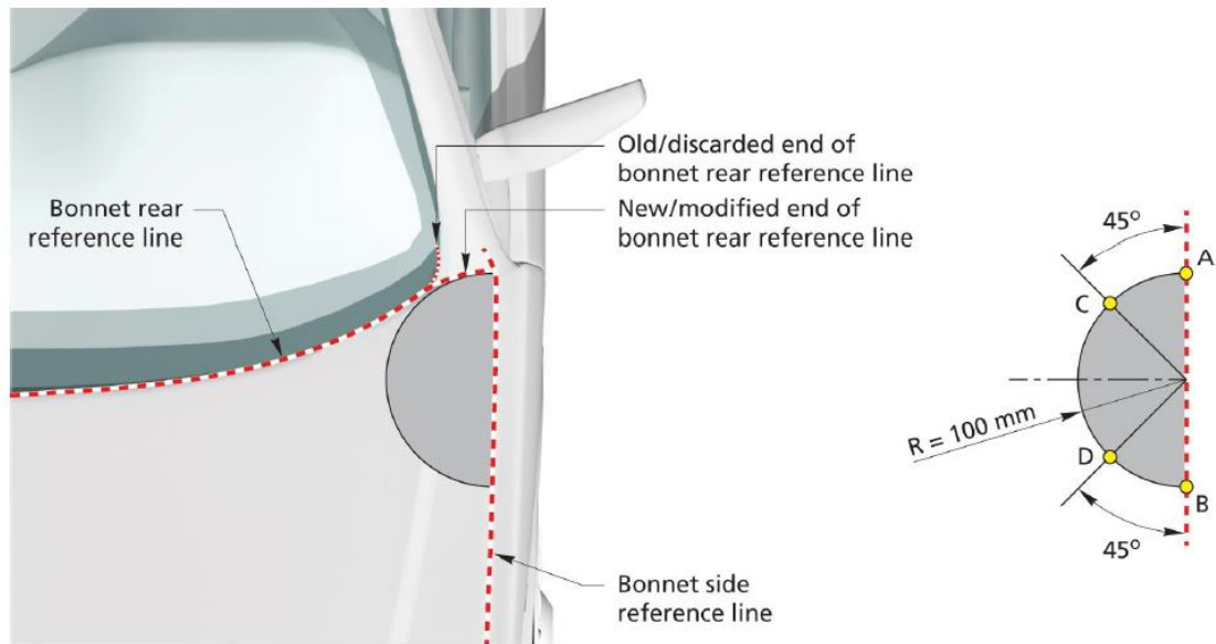
Figure 8: Bonnet rear reference line template and extension
