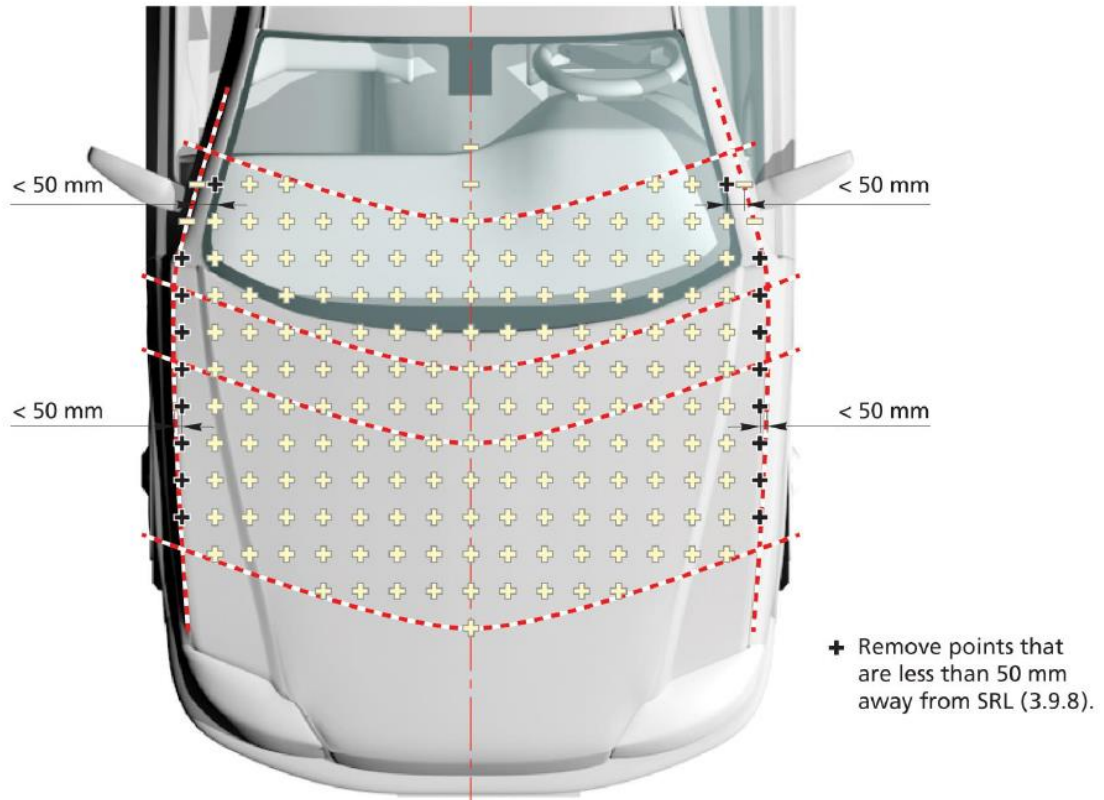
Figure 19: Deleting grid points that are less than 50mm away from side reference line
