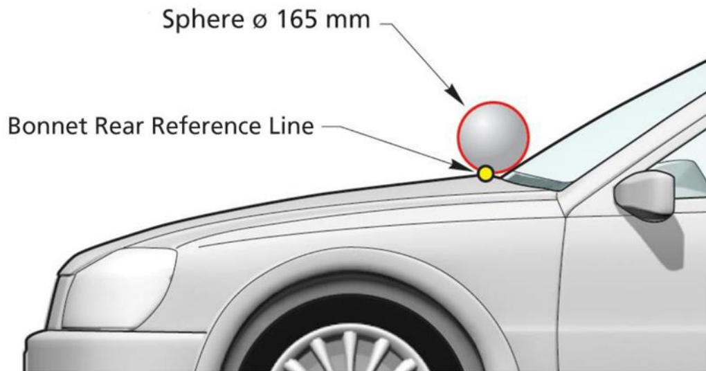
Figure 7: Determination of the bonnet rear reference line
