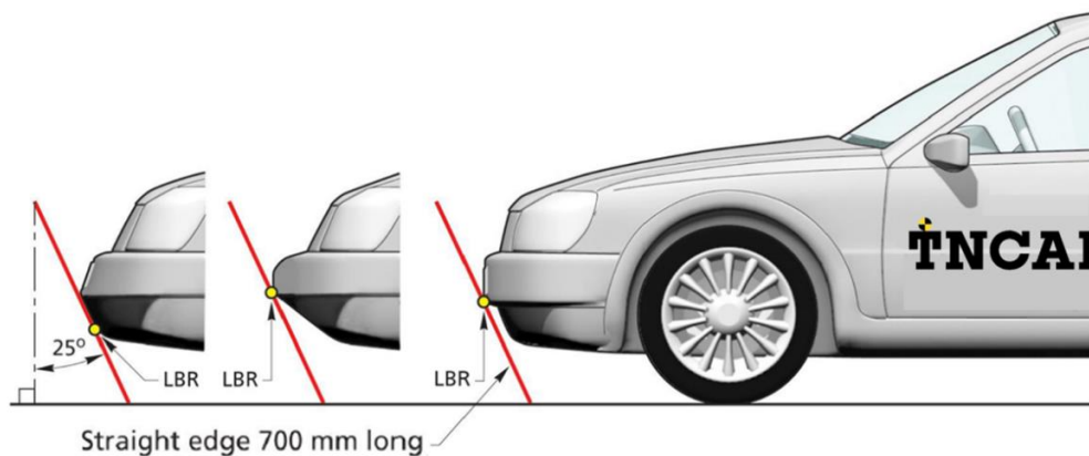
Figure 13: Determination of the Lower Bumper Reference Line
