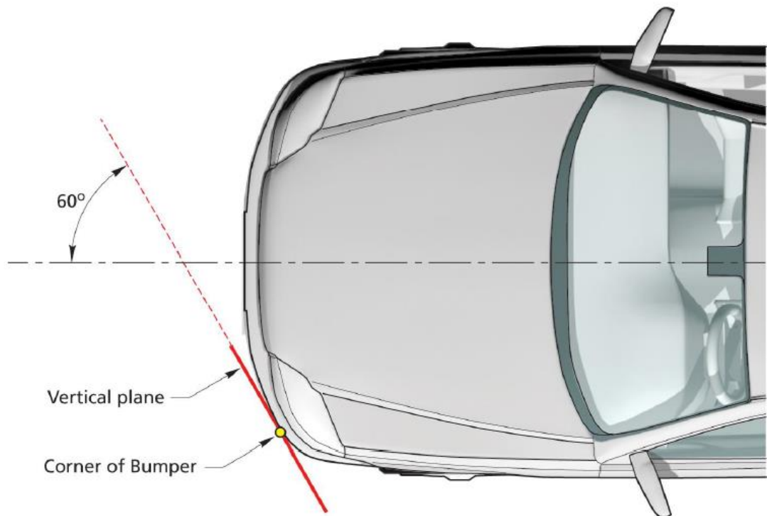
Figure 14 Determination of bumper corner
