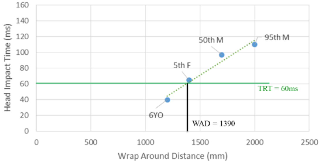
Figure 1: Wrap Around Distance (WAD) vs Head Impact Time (HIT)
